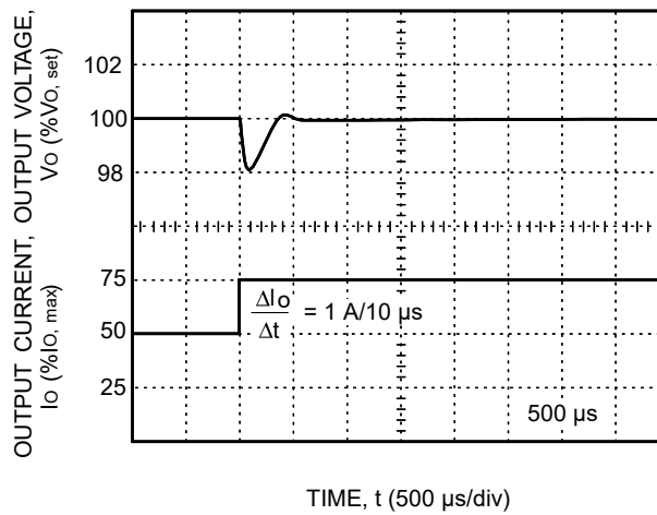
Figure 16. JW030A-M, Typical Output Voltage for a Step Load Change from 50% to 75%
