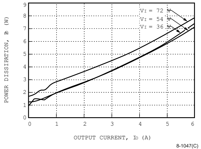
Figure 31. JW030A-M Power Dissipation vs. Output Current
