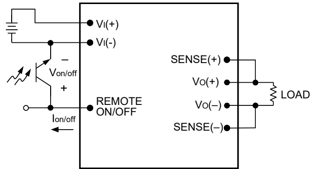
Figure 23. Remote On/Off Implementation
