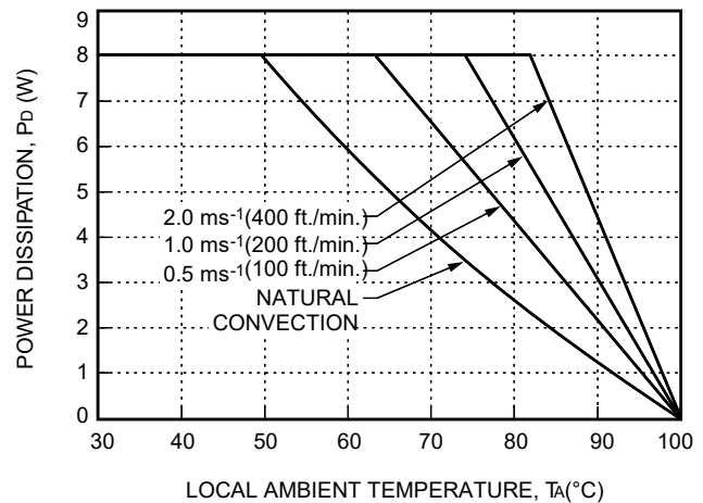
Figure 34. Forced Convection Power Derating with No Heat Sink; Either Orientation
