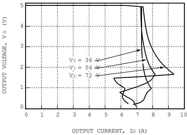
Figure 6. JW030A-M Typical Output Characteristics
