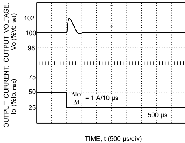
Figure 18. JW030A-M, Typical Output Voltage for a Step Load Change from 50% to 25%
